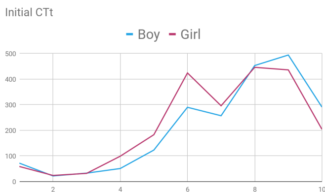
Figure 5.1.3.a. Students' estimation of how well they believe they performed on the CTt
